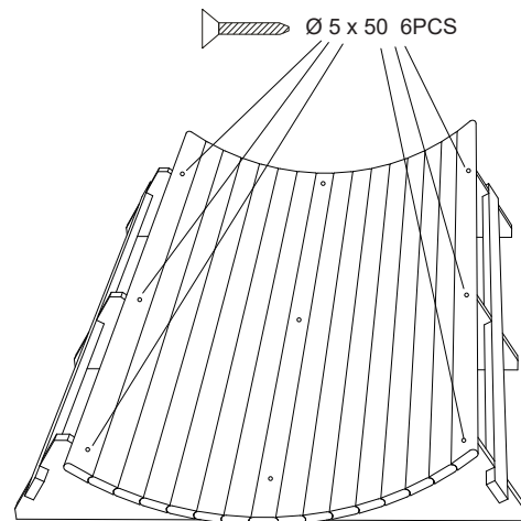
Under slat
