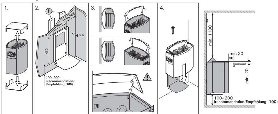
Installation diagram of sauna stove
